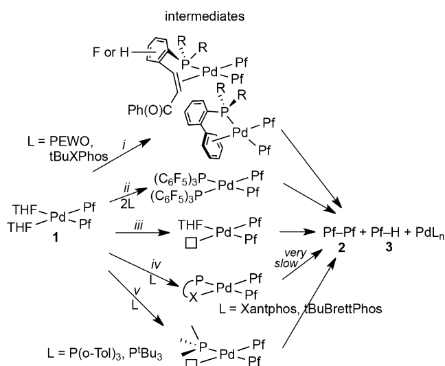
Scheme 2. Reaction \text{Pd}^{\text{II}} intermediates and final products formed by reaction of 1 with the different ligands in Table 1.
