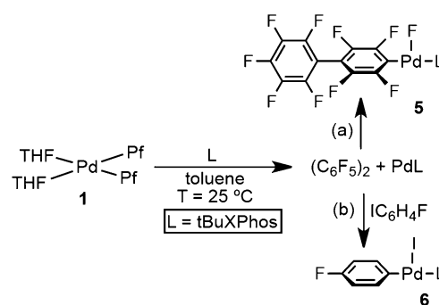
Scheme 5. Synthetic potential of complex 1 as a precursor of the \text{Pd}^0\text{L} catalyst.
