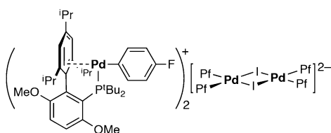
Scheme 4. Cation and anion structures of the ionic complex [\text{Pd}(\text{C}_6\text{H}_4\text{F})(t\text{BuBrettPhos})]_2[(\mu\text{-I})_2(\text{PdPf}_2)_2] ( 4 ). See X-ray diffraction structure in the Supporting Information.
