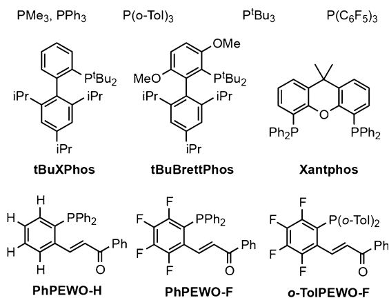
Scheme 1. Phosphine ligands used in this work.
