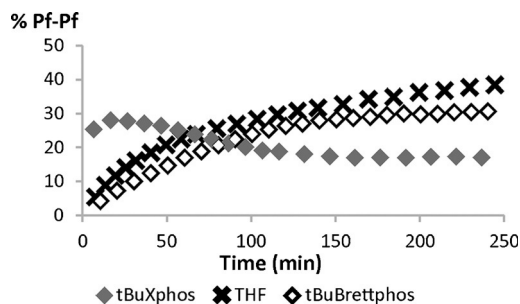
Figure 1. Percentages of Pf-Pf not adding ArI promoted by some ligands in Scheme 1. The line for THF is kept as shown in Figure 2 for reference.
