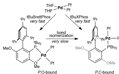
Scheme 3. Different coordination behavior of t BuXPhos and t BuBrettPhos.
