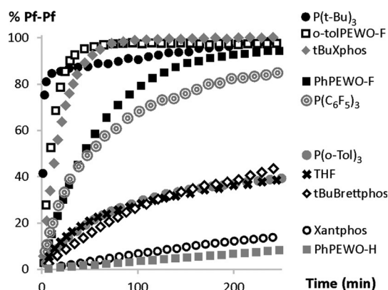
Figure 2. Percentages of Pf (relative to the starting material 1 ) obtained as Pf-Pf promoted by ligands in Scheme 1. All at 25 °C, in toluene. L:1 = 2:1.
